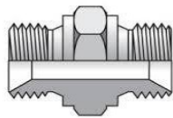
BSSP adapter
